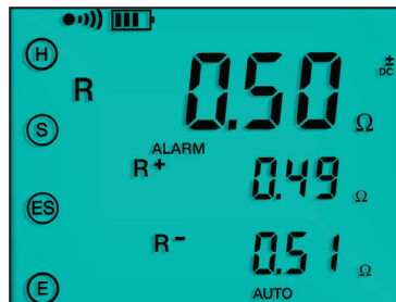
The 4-Point test shows lead connections, Continuity test results, test voltage and current
